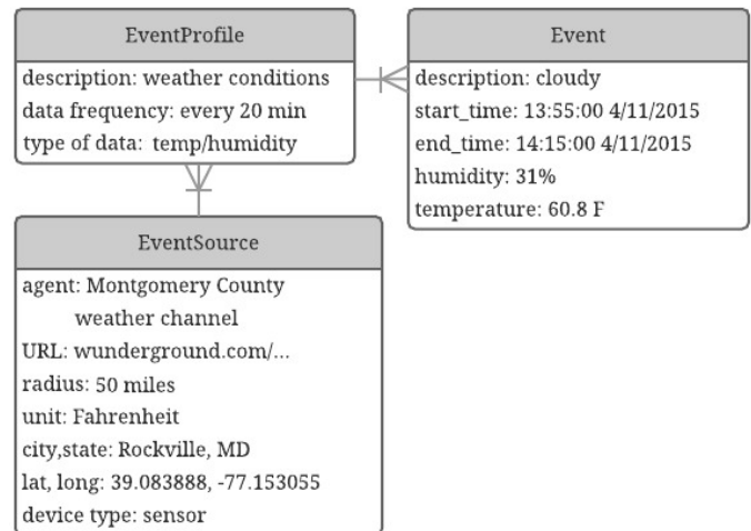
Fig. 4. Weather condition metadata in our event model
