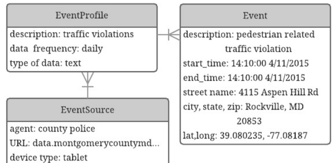
Fig. 5. Traffic violation metadata in our event model
