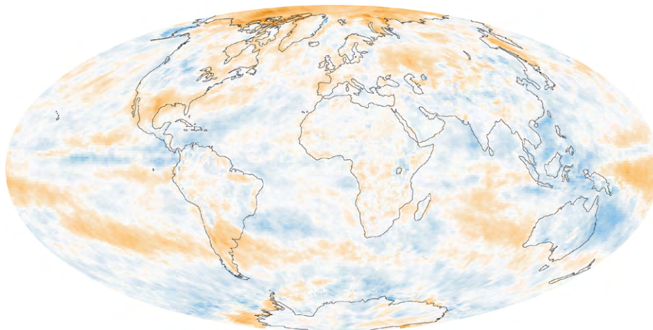
Figure 1. NASA Earth Observatory image by Robert Simmon based on data from CERES satellite. ( earthobservatory.nasa.gov/IOTD/view.php?id=84499 )
