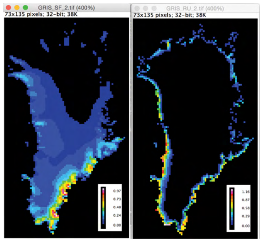
Figure 3. Screenshot of a comparison of snowfall (left) and runoff data (right). (Figure provided by the authors). The color bars show the average annual water equivalent (2005-2016) of snowfall or runoff in units of km 3 /year.
