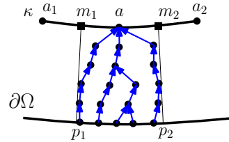
Fig. 3: A discrete chord.
