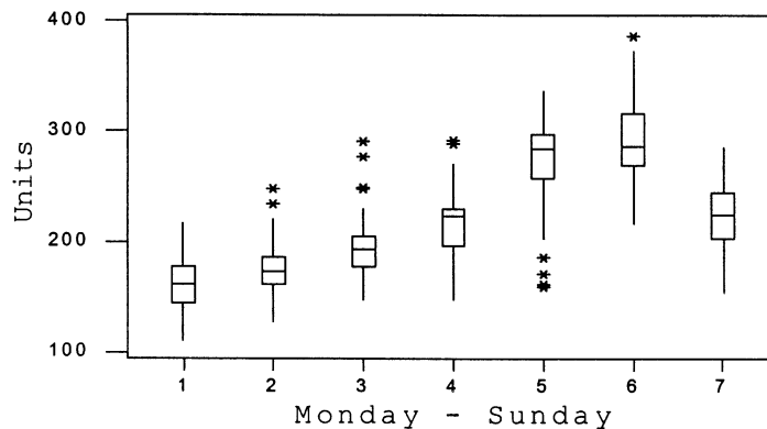
Fig. 3. Box-and-whisker plot (Monday through Sunday) for the daily demand of a perishable ingredient.
