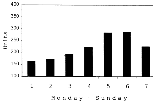
Fig. 2. Median daily demand (Monday through Sunday) of a perishable ingredient.
