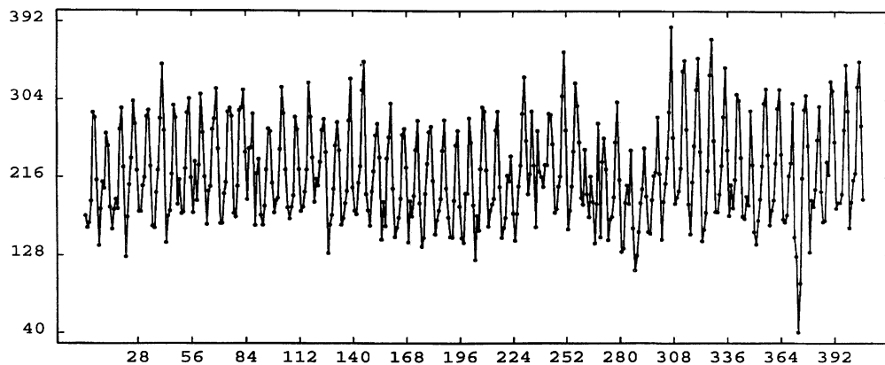
Fig. 1. Daily demand of a perishable ingredient for a fast-food restaurant (4/7/97 ~ 5/18/98).
