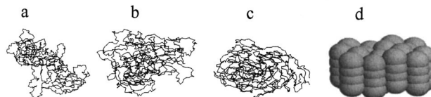
FIG. 7. Examples of self-avoiding walks of length 1000 generated with different sampling probability function e^{-E'(c)/T'} using different (T', c) values. (a) Conformations generated with (T', c) = (1.0, 0.0) ; (b) (T', c) = (0.67, 0.0) ; (c) (T', c) = (0.1, 0.6) ; (d) Approximate maximally compact conformation.
