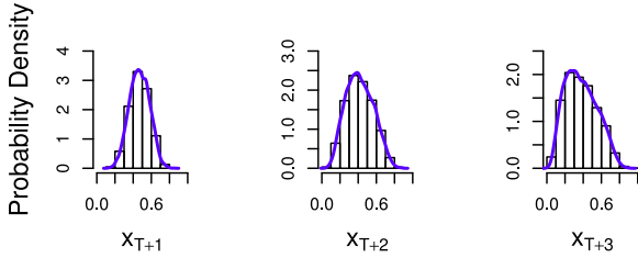
Fig. 2. Posterior predictive distributions p(x_{T+h} | x_{1:T}) with h = 1, 2, 3 .
