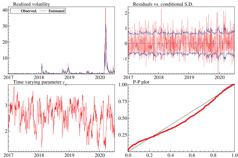
Figure 1. Modeling S&amp;P 500 realized volatility using GARMA-GARCH model
